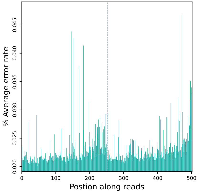
Error rate distribution along reads (R10306)
